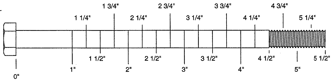
5/16" HEX BOLT
